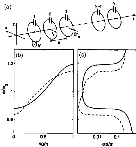
Fig. 11.5 (a) One-dimensional axial structure of capacitively loaded loops. (b) Dispersion curves for the one-dimensional axial structure: nearest-neighbor interactions only ( solid line ), interactions between five neighbors ( dashed line ). Reprinted with permission from [51].
