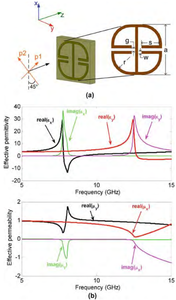
Fig. 14.24 (a) The ELC unit for polarization design: a = 3.6\text{mm} , w = 0.2\text{mm} , g = 0.2\text{mm} , s and r are variables. The copper thickness is 0.035\text{mm} and the substrate thickness is 0.75\text{mm} . (b) The retrieved permittivity and permeability for the optimized ELC from 5 to 15 GHz. Copyright ©2008 American Institute of Physics.
