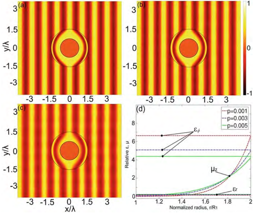
Fig. 2.4 The distributions of magnetic fields inside circular cloaks with inner radius 0.025 m ( 0.75\lambda_0 ), and, outer radius 0.05 m ( 1.5\lambda_0 ). (a) The half focus p = 0.001 m, (b) the half focus p = 0.003 m, (c) the half focus p = 0.005 m, and (d) the distributions of \mu_z , \varepsilon_\phi , and \varepsilon_r components in the cloaking region.
