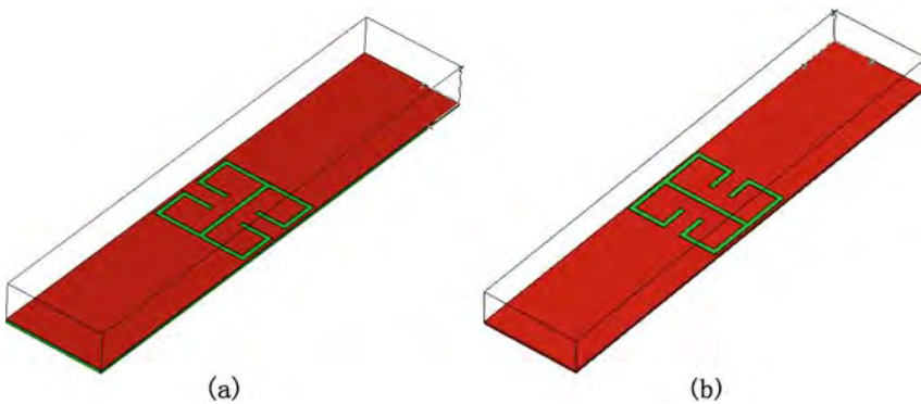
Fig. 14.14 Simulation setups for the anisotropic CELC unit cell where the plane waves are incident from two orthogonal directions.
