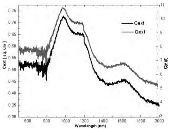
Fig. 12.8 Extinction cross section of bow tie structures prepared on ITO/glass substrate. The actual geometric cross section is 0.0672\text{ }\mu\text{m}^2 , while a value 10 times geometric cross section is observed by the detector.
