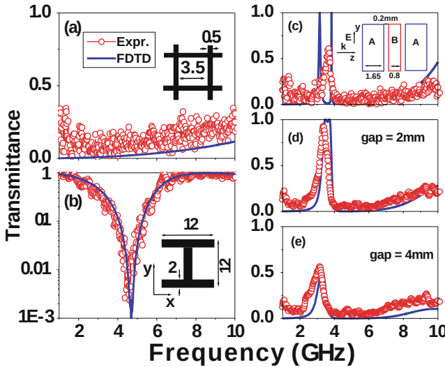
Fig. 10.23 Measured (circles) and calculated (lines) transmission spectra through a single “B” layer (a) and a single “A” layer (b). The unit cell structures of “B” and “A” layers are shown in the insets with all lengths measured in mm, and please refer to Ref. [58] for more details of the structure. (c–e) Measured (circles) and calculated (lines) transmission spectra of the ABA structure with different air gaps between layers A and B. Reproduced from Ref. [58] with the permission of American Physical Society.
