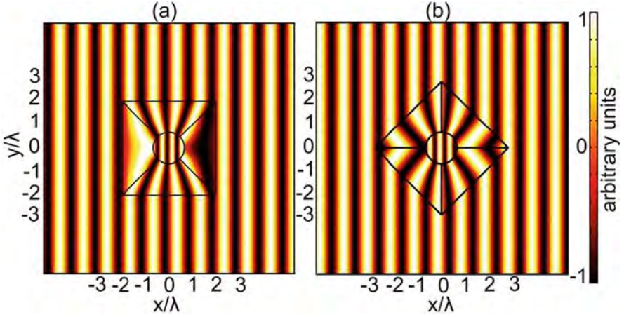
Fig. 2.8 The distributions of electric fields for a non-conformal concentrator with different inner and outer boundaries. (a) The square outline of the concentrator is parallel to the x -axis. (b) The square outline of the concentrator is rotated by \pi/4 with respect to the x -axis.
