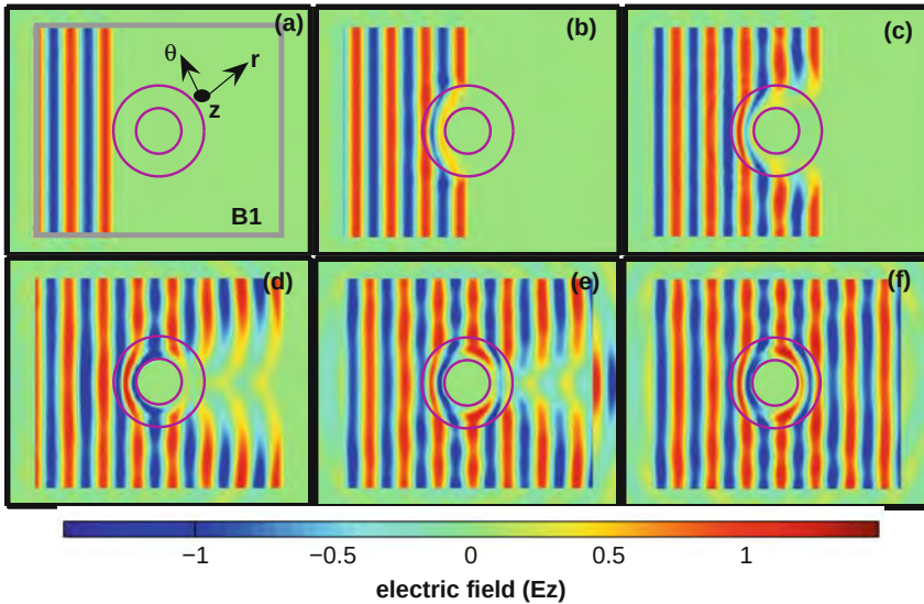
Fig. 9.5 (Color online) (a) The setup of the system and the distribution of the electric field at different moments during the process. Parameters are chosen as A_r = 0.4 , A_\theta = 1.6 , A_z = 0.4 (in the position where \epsilon_z < 1 ) or A_z = 1.6 (where \epsilon_z > 1 ), and \gamma = 0.012\omega_0 . (a) t = 2.28T ; (b) t = 3.60T ; (c) t = 4.92T ; (d) t = 7.20T ; (e) t = 9.00T ; (f) stable state. T is the period of the incident EM wave.
