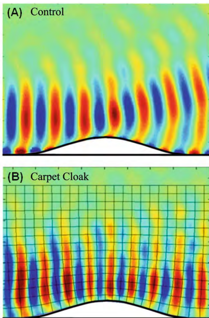
Fig. 6.10 Two-dimensional field mapping (E-field) of the perturbation and ground-plane cloaked perturbation, illuminated by the waves from the left side (a) perturbation, (b) ground-plane cloaked perturbation. The grid pattern indicates the quasi-conformal mapping of the transformation optics material parameters. From Ref. [4].
