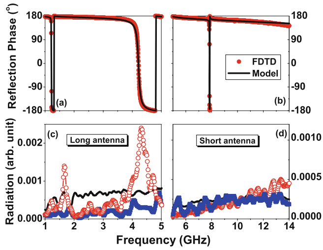
Fig. 10.10 (a), (b) Reflection phase change on the surface of our composite, calculated by FDTD simulation (solid symbols) and an effective medium model (solid lines), for x -polarized incident wave. (c), (d) Measured forward radiation spectra for free antennas (solid line), antennas on the surface of a metal sheet (solid squares), and on the surface of the composite (open circles). The fractal's first-level line is perpendicular to the antennas' wires. Reproduced from Ref. [57] with the permission of American Institute of Physics.
