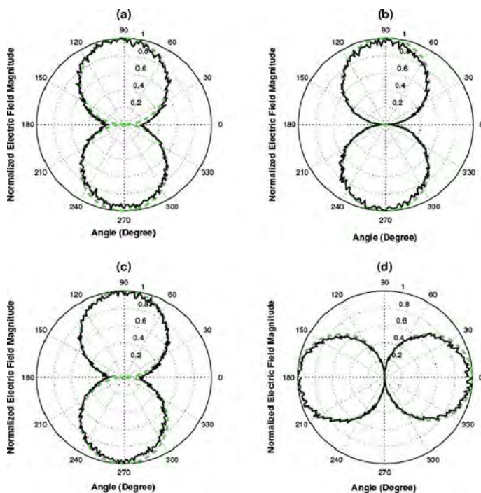
Fig. 14.32 Measured polarization patterns (solid line) and ideal polarization patterns (dashed line) of the transmitted waves at 8.0 GHz (a), 8.5 GHz (b) and 9.0 GHz (c) compared with measured polarization pattern of the incident waves at 9.0 GHz (d). Copyright © 2009 Optical Society of America.
