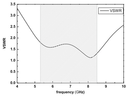
Fig. 13.21 Simulated VSWR of proposed antenna (when gap = 0.4 mm). Shaded area depicts the working band.
