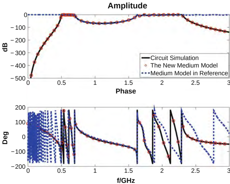
Fig. 1.8 The transmission coefficients of a 10-cell periodic structure computed by circuit simulations and effective medium models. (a) Amplitude. (b) Phase.
