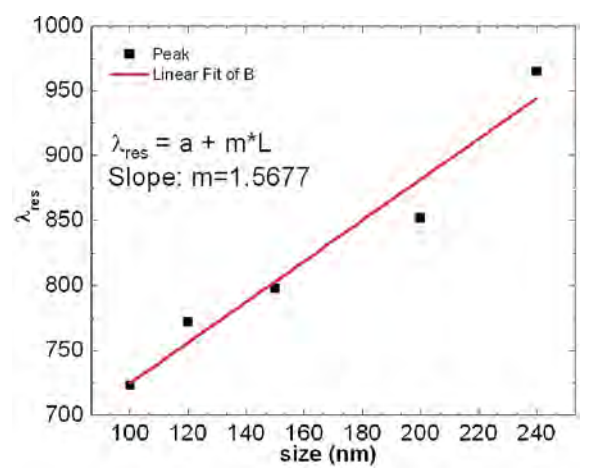
Fig. 12.9 The resonant wavelength vs. the size of the bow tie. The resonant wavelengths are obtained from the peaks transmission spectra, which are plotted by dots , and the line is the linear fitting. The fitting parameters are shown in the inset table.
