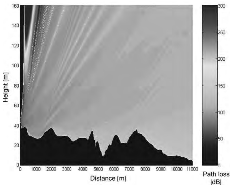
Figure 6.27: Predicted path loss over irregular terrain using parabolic equation
