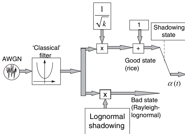
Figure 14.11: Two-state Lutz model of narrowband mobile satellite fading
