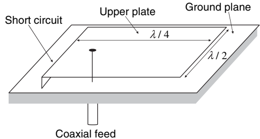
Figure 15.7: Planar inverted-F antenna
