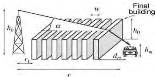
Figure 8.8: Geometry for the flat edge model
