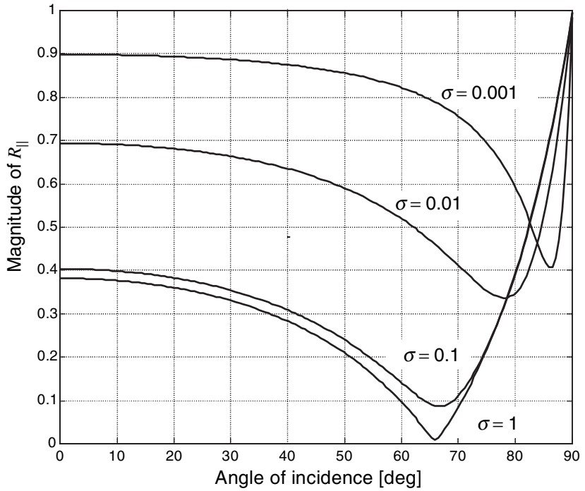
Figure 3.6: Pseudo-Brewster angle: R_{\parallel} never goes to zero ( \varepsilon_{r1} = 1, \varepsilon_{r2} = 5 )
