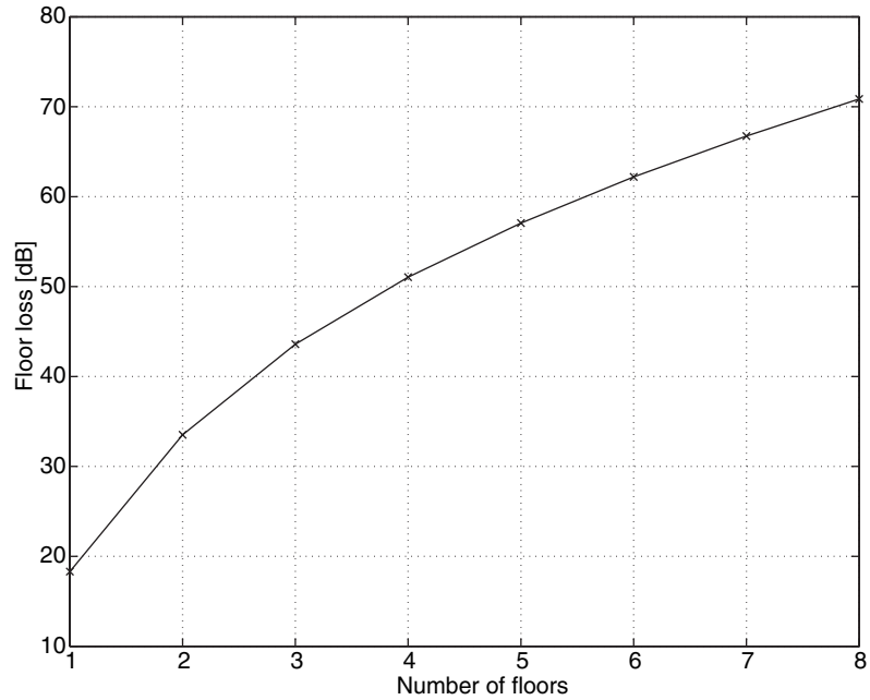
Figure 13.3: Floor loss for COST231 multi-wall model
