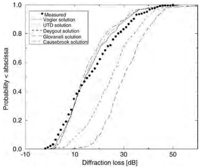
Figure 6.21: First-order statistics for digital broadcasting prediction comparisons [Tzaras, 00]
