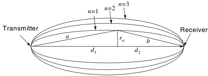
Figure 3.17: Fresnel zones
