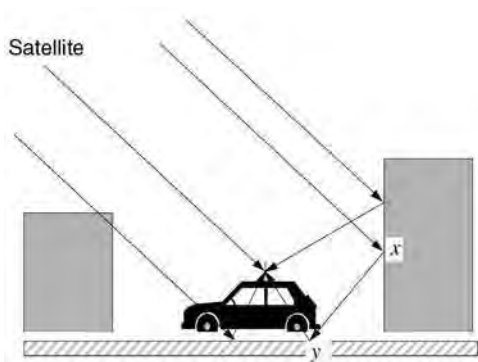
Figure 14.5: Multipath propagation
