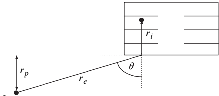
Figure 13.11: Geometry for COST231 line-of-sight building penetration model
