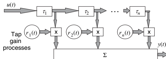
Figure 11.6: Wideband channel model
