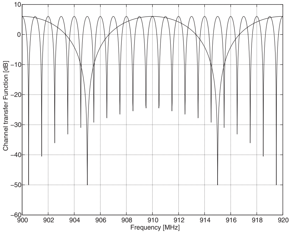
Figure 11.3: Transfer function of two-path channel: relative path delays 1 \mu\text{s} and 0.1 \mu\text{s}
