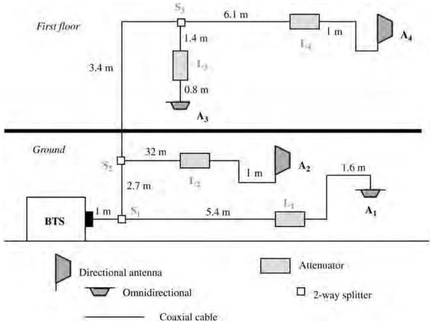
Figure 13.32: Passive indoor distributed antenna system for example 13.2
